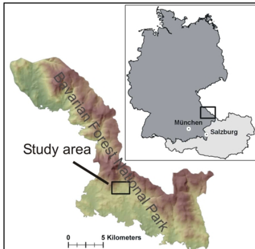
Figure 1. Study area location within the Bavarian Forest National Park
