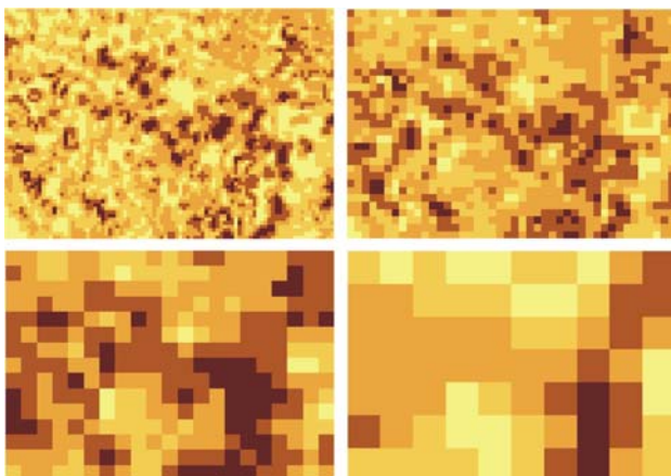
Figure 4. Resulting height standard deviation based on moving windows at four different scales. Window sizes are 5m (upper left), 10m (upper right), 20m (lower left), 40m (lower right). Dark colours indicate higher values.
