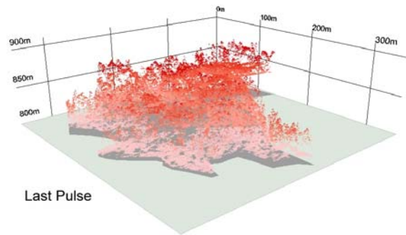
Figure 2. LiDAR point data (x,y,z-triples) imported in a GIS as seen from the side. Colour intensities represent high z-values, for both the first pulse and the last pulse signals.
